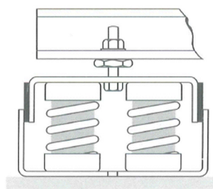
Assembly with leveling
